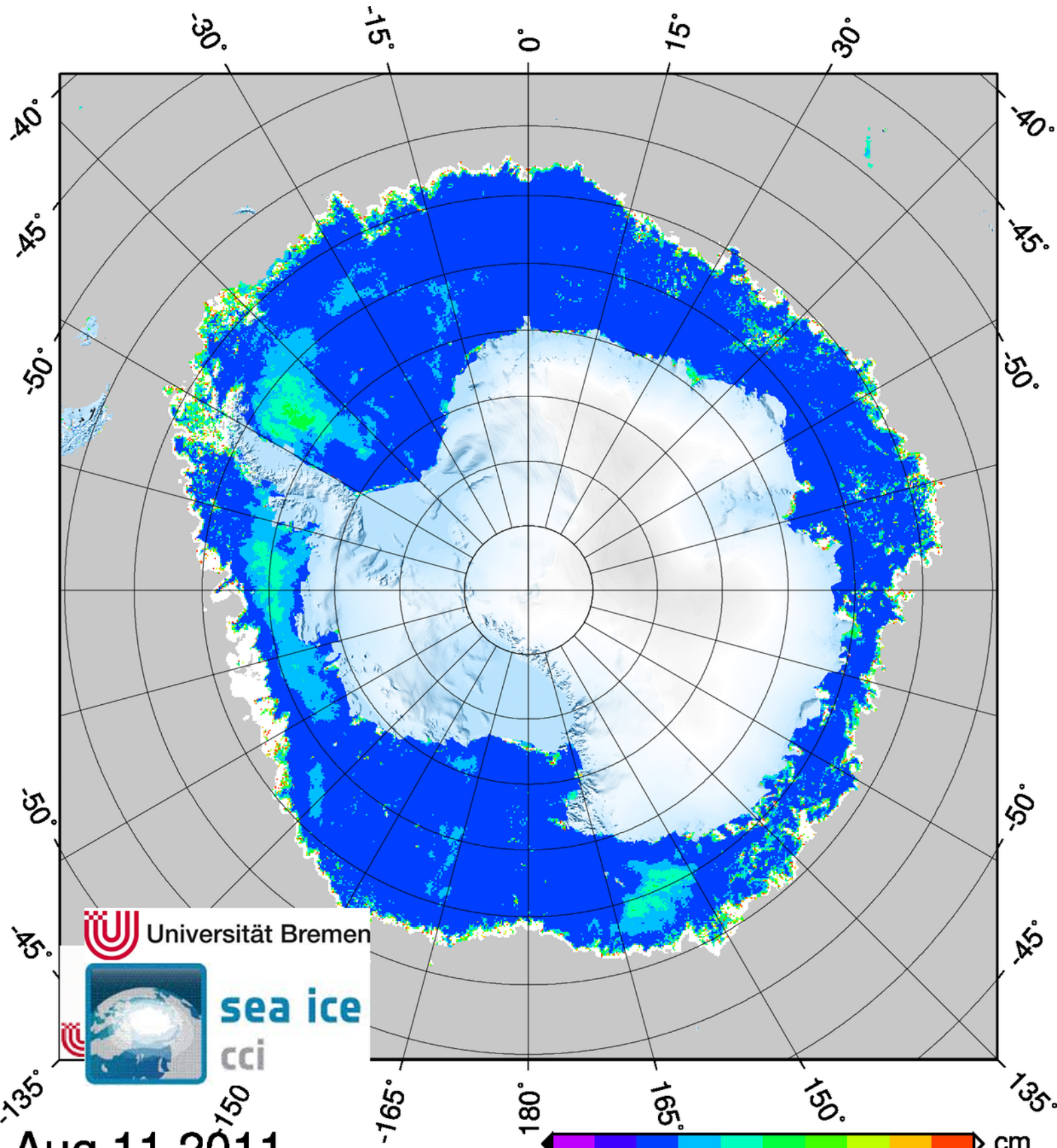
Error Snow on sea ice v1.0Grid 12.5 km, Geolocation_UB Error of Snow Depth cm
