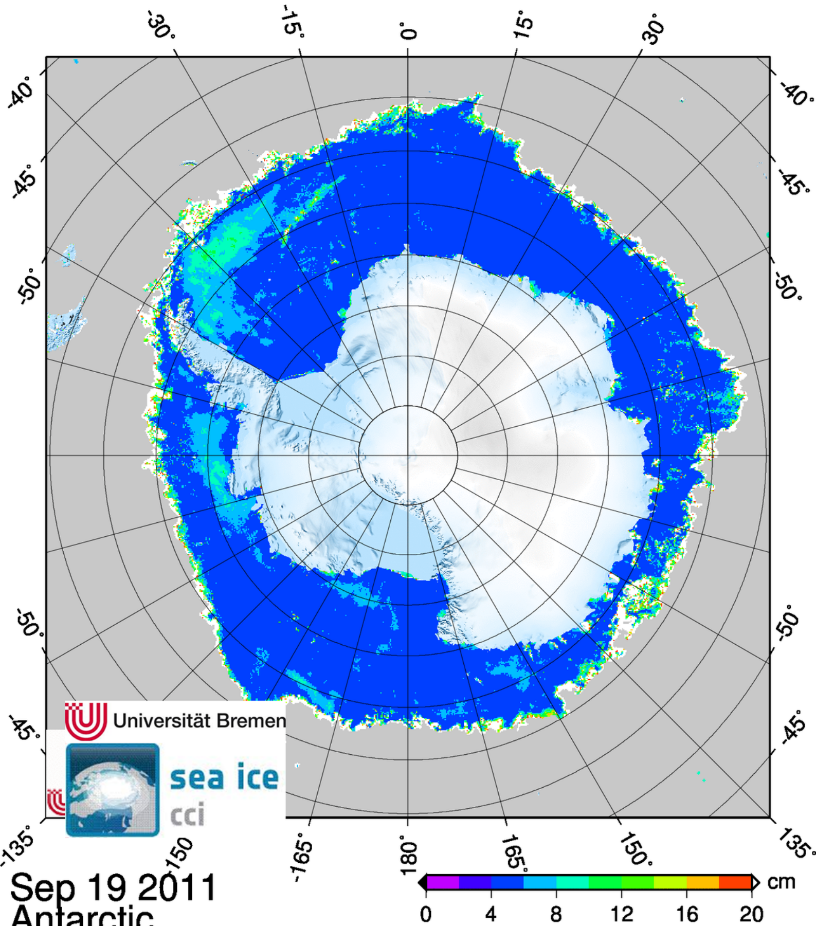
Error Snow on sea ice v1.0 Grid 12.5 km, Geolocation_UB
